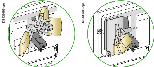
Toggle locking using padlocks and an accessory: Removable device
