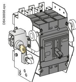
Chassis locking in the connected position
