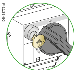
Rotary-handle locking using a keylock
